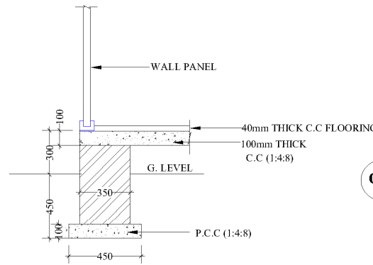
TYPICAL FOUNDATION DETAIL BY BRICK MASONRY / STONE MASONRY
