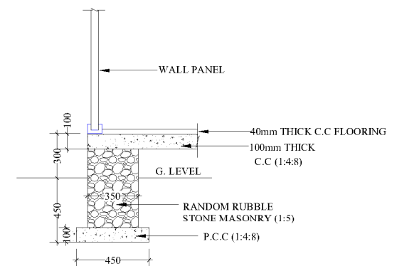
TYPICAL FOUNDATION DETAIL BY BRICK MASONRY / STONE MASONRY
