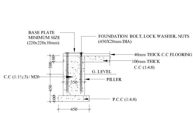
TYPICAL DETAIL FOR BOLT FOUNDATION
